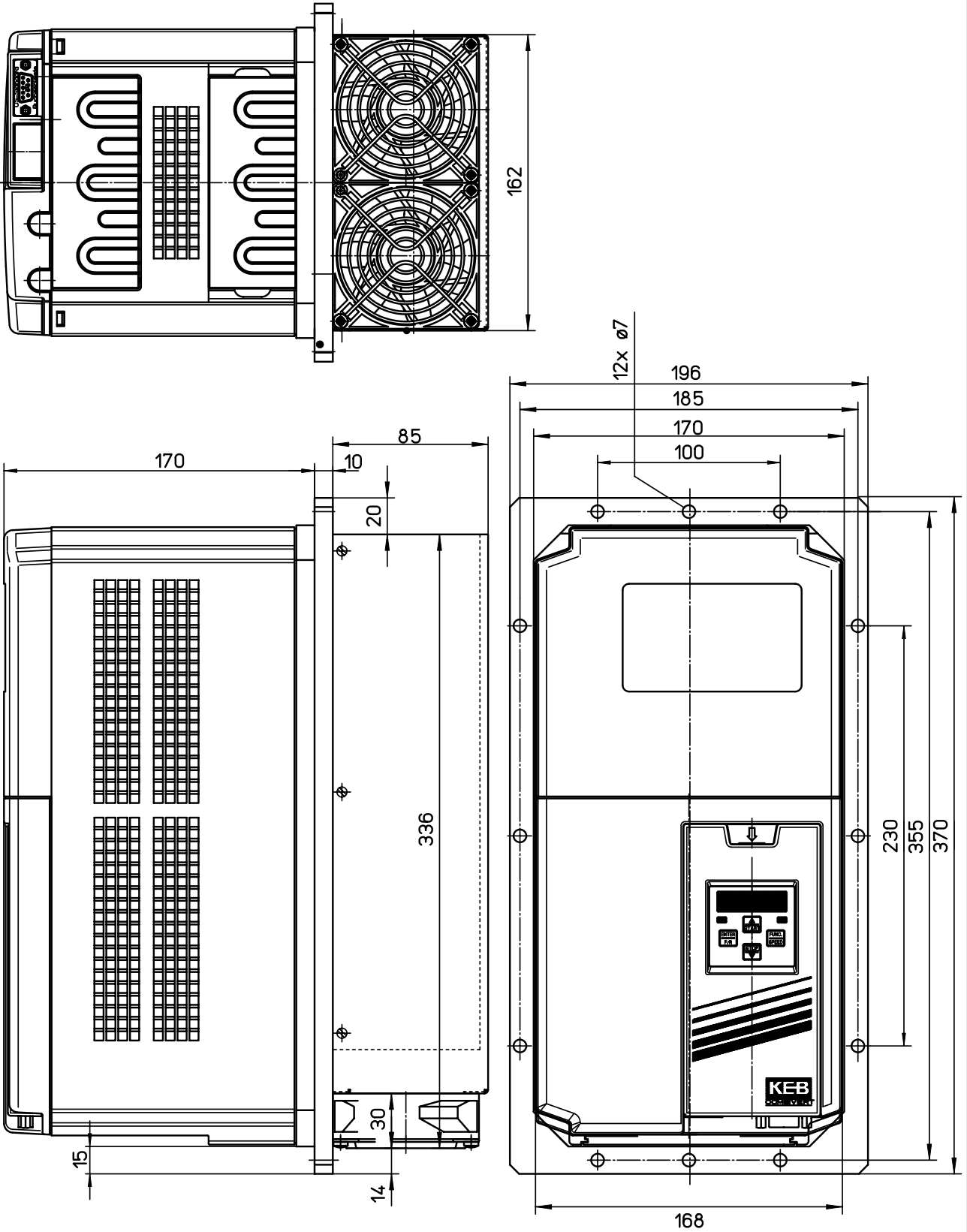
Dimensions through-mount version air-cooled (with fan)
