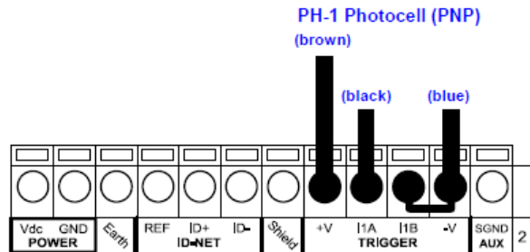
Figure 14 – PH-1 External Trigger Using CBX Power
