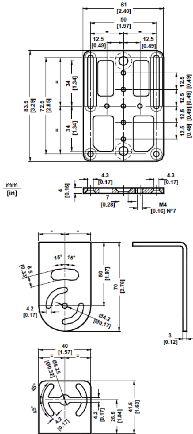
Figure 5 – Mounting Bracket Overall Dimensions
