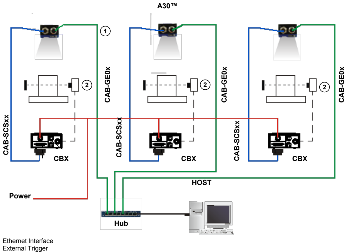
Figure 46 - Ethernet Network Layout
