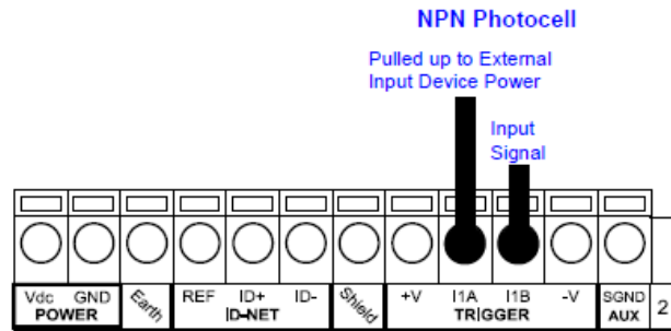
Figure 17 - NPN External Trigger Using External Power
