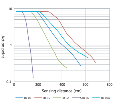
Polarized reflection
