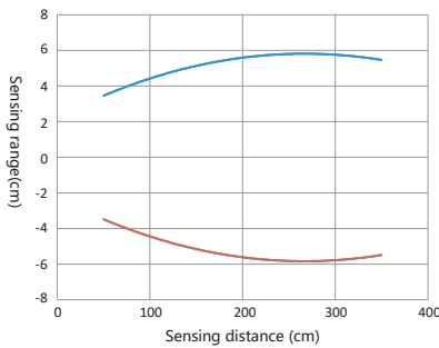
Polarized reflection
