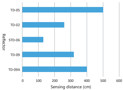
Polarized reflection
