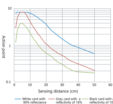
Diffuse reflection
