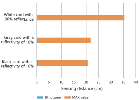
Diffuse reflection
