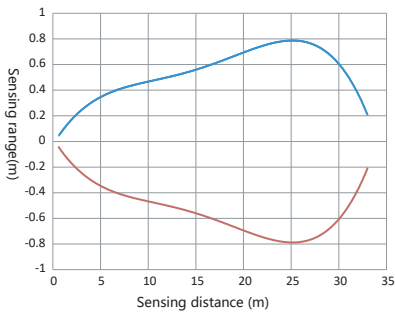
Through beam
