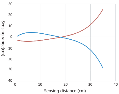
Diffuse reflection
